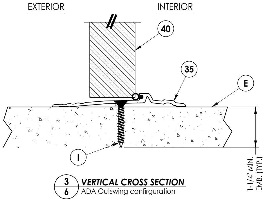
1 6 VERTICAL CROSS SECTION Outswing configuration
