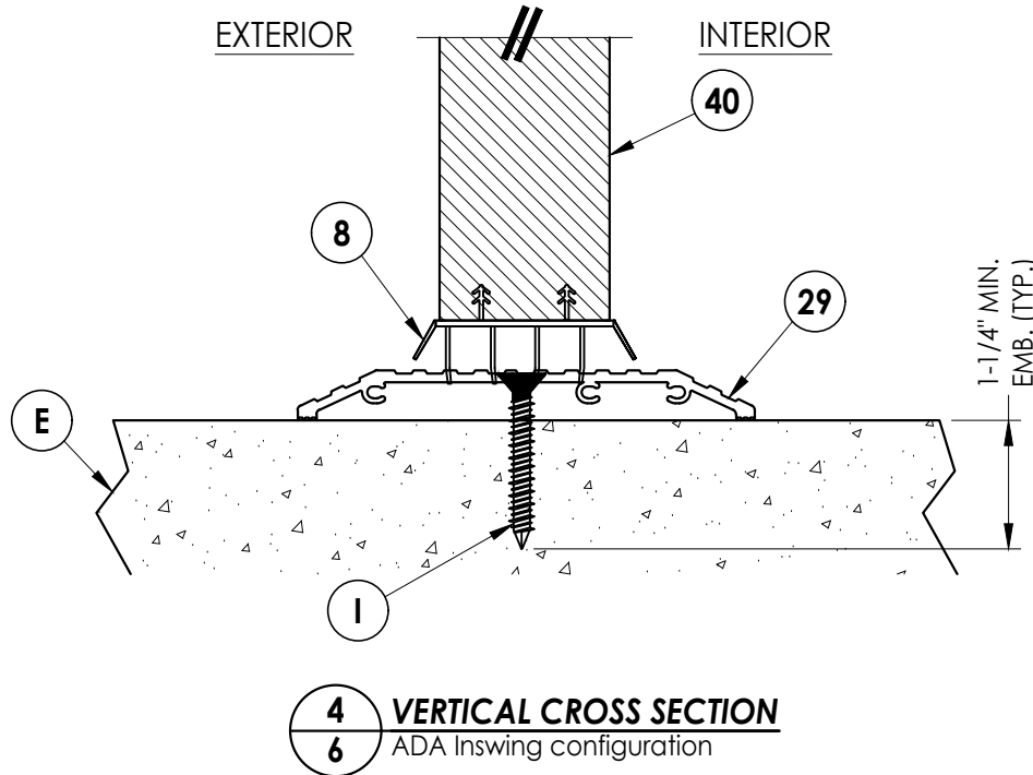
2 6 VERTICAL CROSS SECTION Inswing configuration
