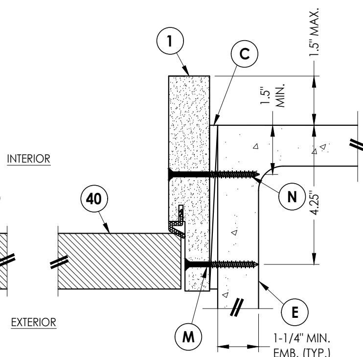
4 HORIZONTAL CROSS SECTION 7 Shown Direct to Masonry Outswing only w/ 6-9/16" jamb
