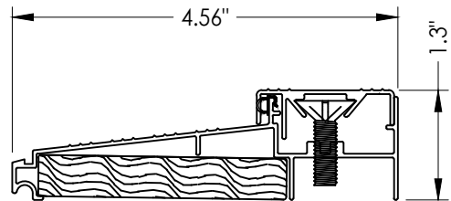
37 INSWING THRESHOLD DLP (ISC)
